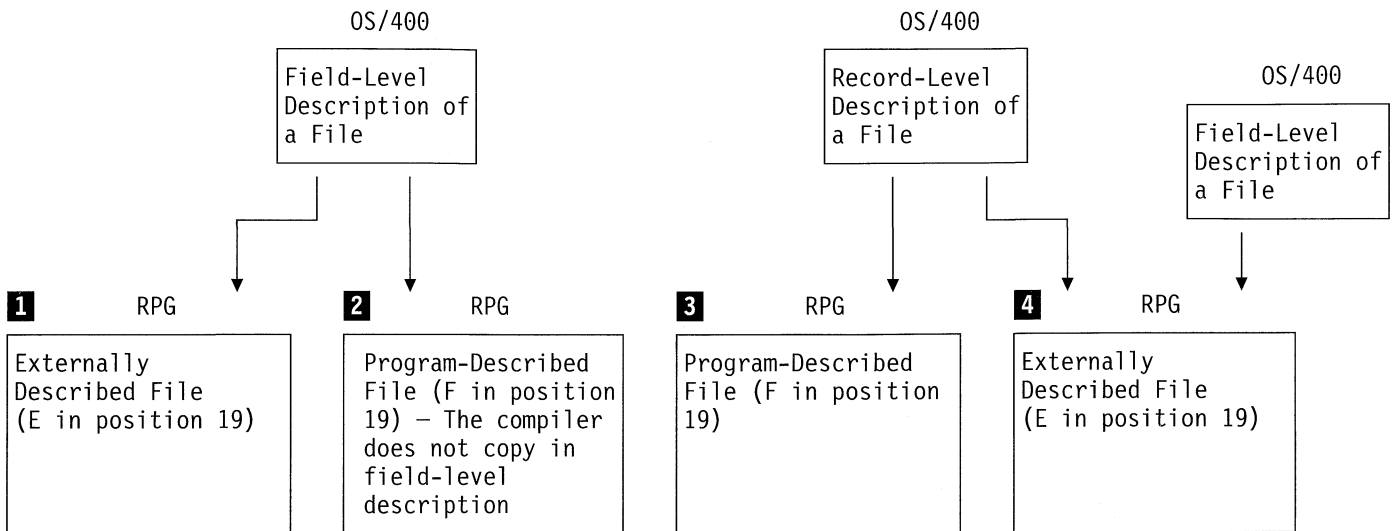
Figure 35. Typical Relationships between an RPG/400
