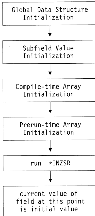
Figure 118. Order of Initialization in an RPG/400 Program.
