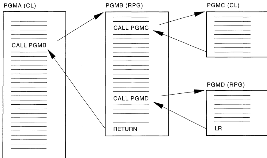
Figure 128. Calling RPG/400 programs and CL programs
