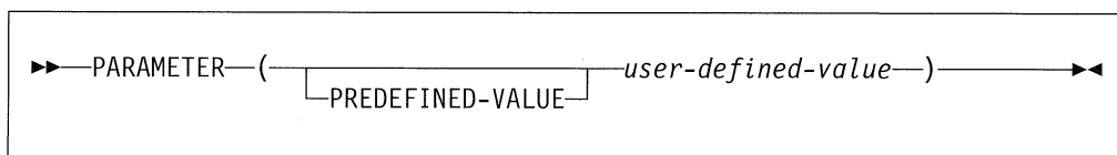
Figure 1. Structure of a Syntax Diagram
