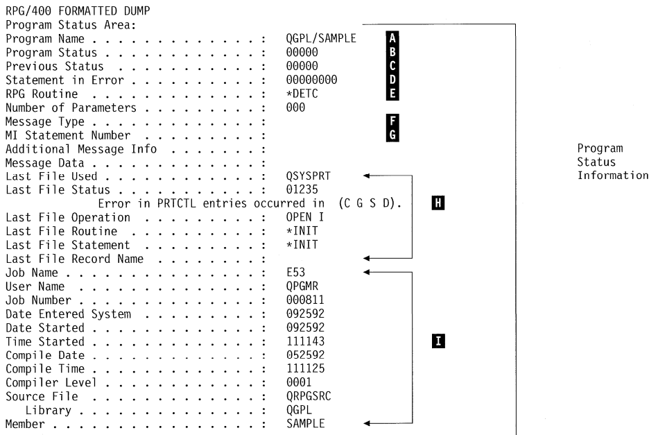
Figure 32 (Part 1 of 8). RPG/400 Formatted Dump
