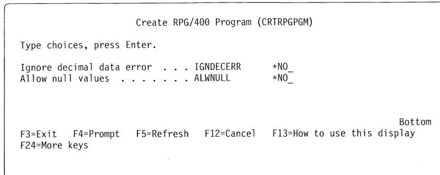
Figure 21 (Part 2 of 2). Third Set of CRTRPGPGM Prompt Screens
